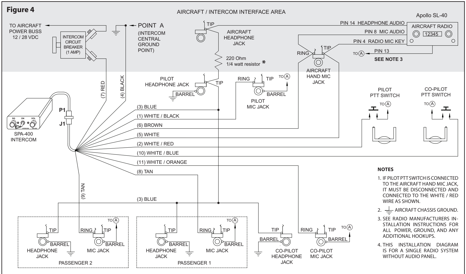
SPA-400 – Apollo SL-40 Radio Installation Wiring Diagram
